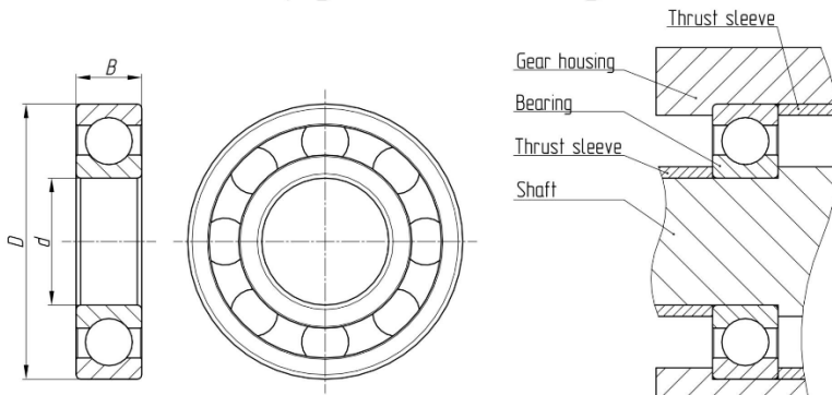
Deep groove ball bearings
